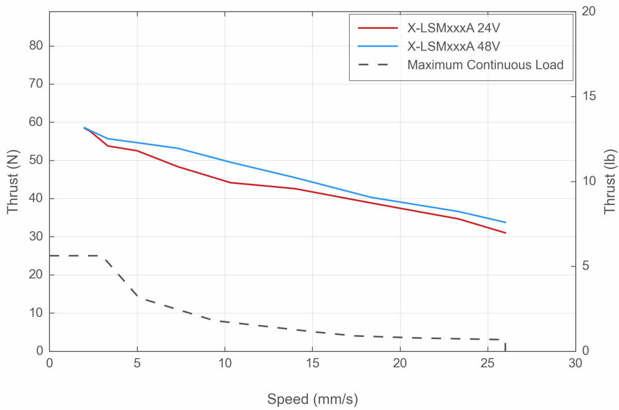
Thrust Speed Performance
